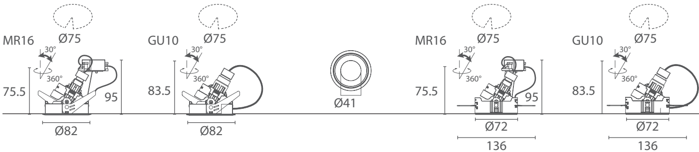
Pinhole Adjustable Trim
