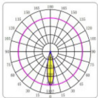
BEAM ANGLE 24°
