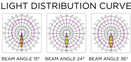
BEAM ANGLE 15° BEAM ANGLE 24° BEAM ANGLE 36°
