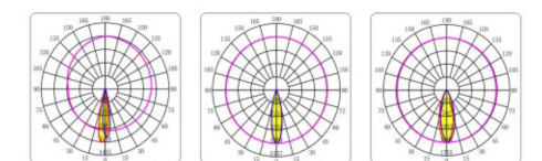
BEAM ANGLE 15° BEAM ANGLE 24° BEAM ANGLE 36°
