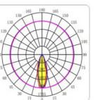
BEAM ANGLE 36°
