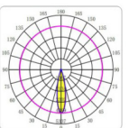
BEAM ANGLE 24°
