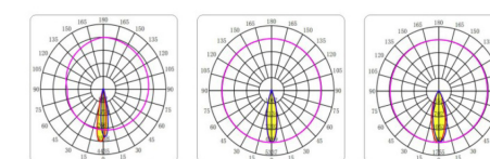
BEAM ANGLE 5° BEAM ANGLE 8° BEAM ANGLE 15°
