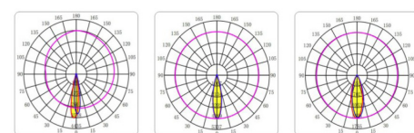
BEAM ANGLE 15° BEAM ANGLE 24° BEAM ANGLE 36°
