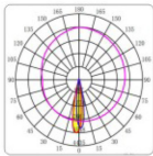
BEAM ANGLE 15°
