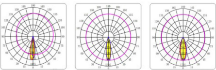
BEAM ANGLE 15° BEAM ANGLE 24° BEAM ANGLE 36°
