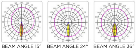
BEAM ANGLE 15° BEAM ANGLE 24° BEAM ANGLE 36°
