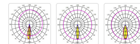
BEAM ANGLE 15° BEAM ANGLE 24° BEAM ANGLE 36°
