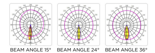
BEAM ANGLE 15° BEAM ANGLE 24° BEAM ANGLE 36°
