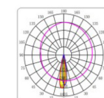
BEAM ANGLE 15°
